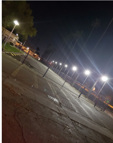
SOLAR AREA LIGHT - 6000 LUMENS Delano High School, CA Fixture Height = 15'
